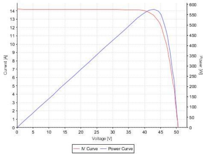
Fig. 5 IV curve of module No.1 Serial number: ASA22190800006
