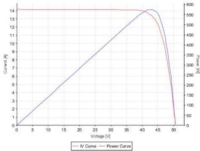
Fig. 6 IV curve of module No.2 Serial number: ASA22190800010
