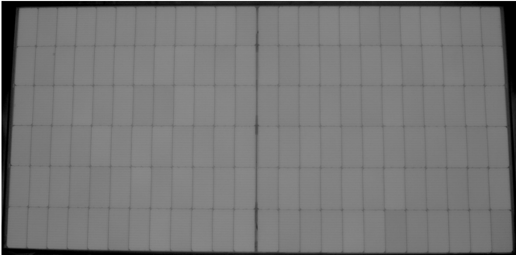
Fig. 8 EL photo of module No.2 Serial number: ASA22190800010
